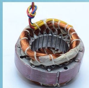
# 3.5 | 25mm 24 SLOT FARATTA HIGH SPEED
