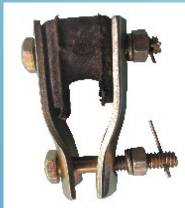
# 14 GAZE HANGING CLAMP # 16 GAZE HANGING CLAMP
