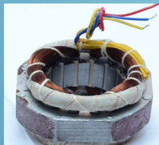
# 3.4 | ORIENT TYPE ROUND HIGH SPEED
